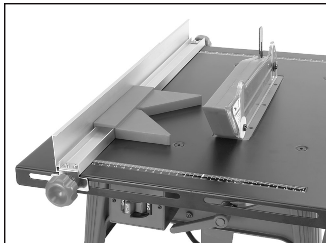
Figure 13. Fence setup for miter cutting.
