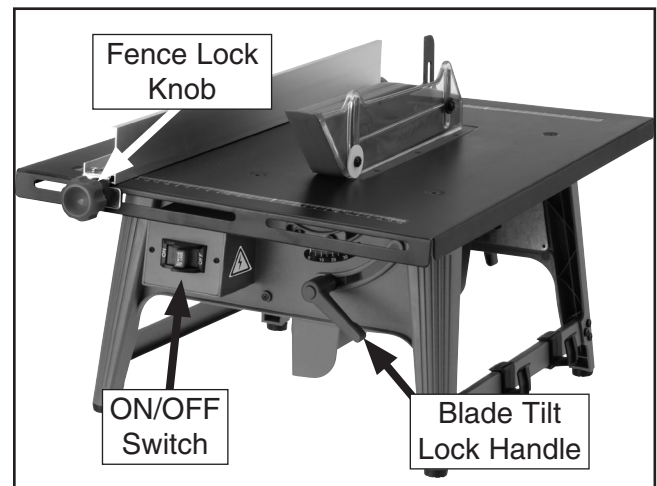
Figure 6. Table saw controls (front).
