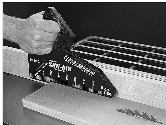
Figure 22. G3445 Precision Saw Tool.
