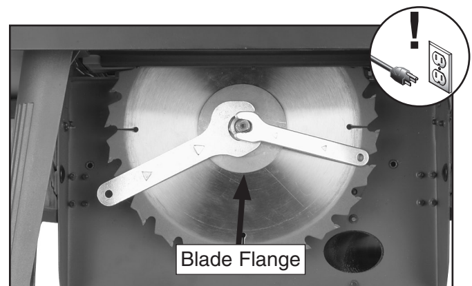
Figure 18. Wrench positions to remove arbor hex nut.
