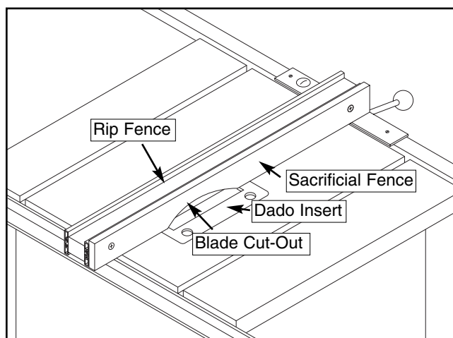
Figure 40. Sacrificial fence.
