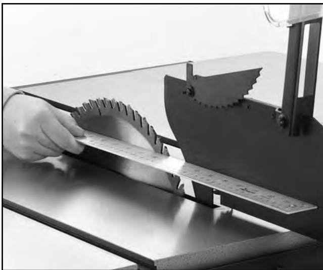
Figure 14. Guard in line with blade.
