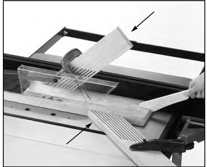
Figure 3. Featherboard.
