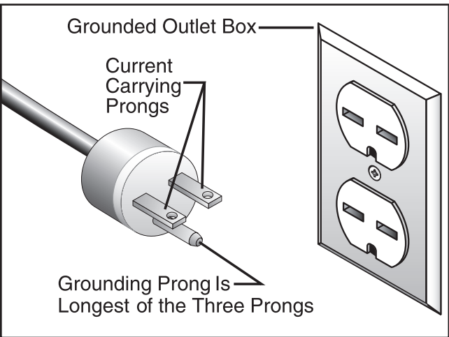
Figure 2. 6-15 plug and outlet.
