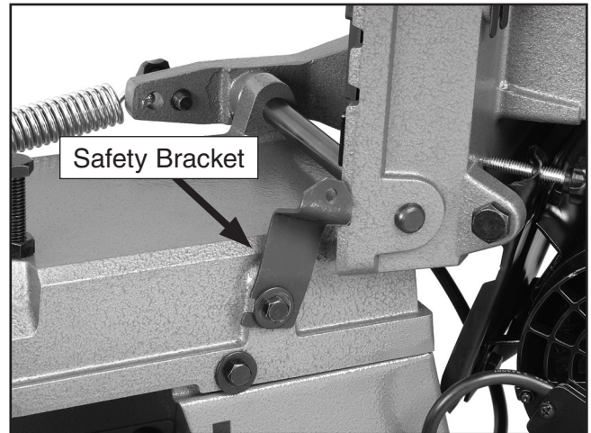
Figure 25. Safety bracket.
